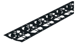
SNAP-FIT RAIL Material: Standard steel blackened Length 960 mm
